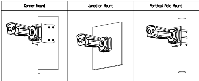
PFA154 Vertical Pole Mount Bracket
